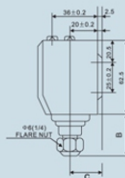
Appearance Drawing
